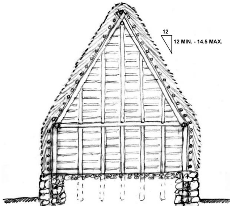
SECTION VIEW
