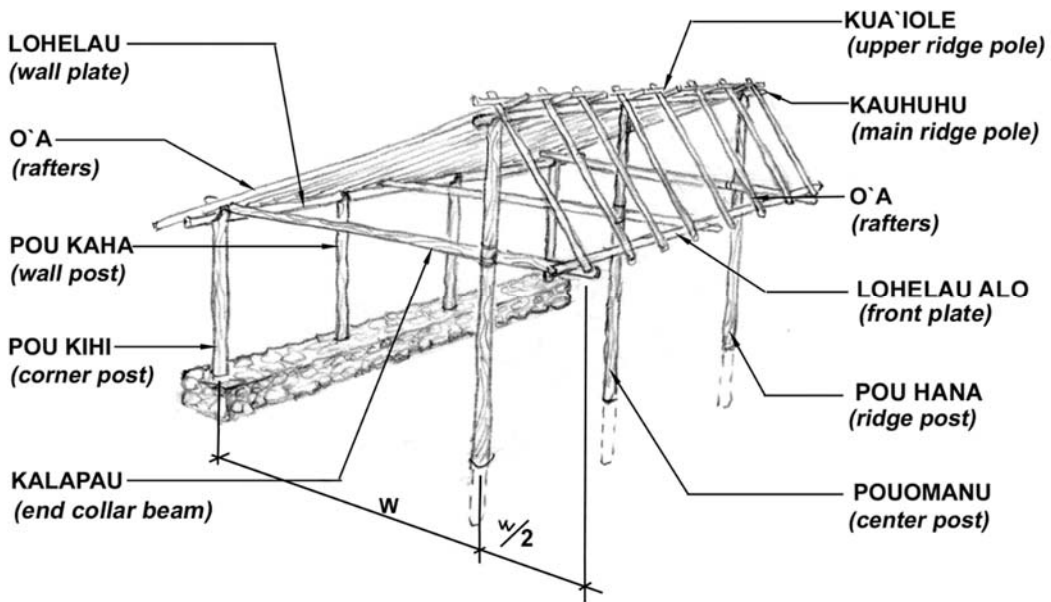
FRAMING SCHEMATIC 2
