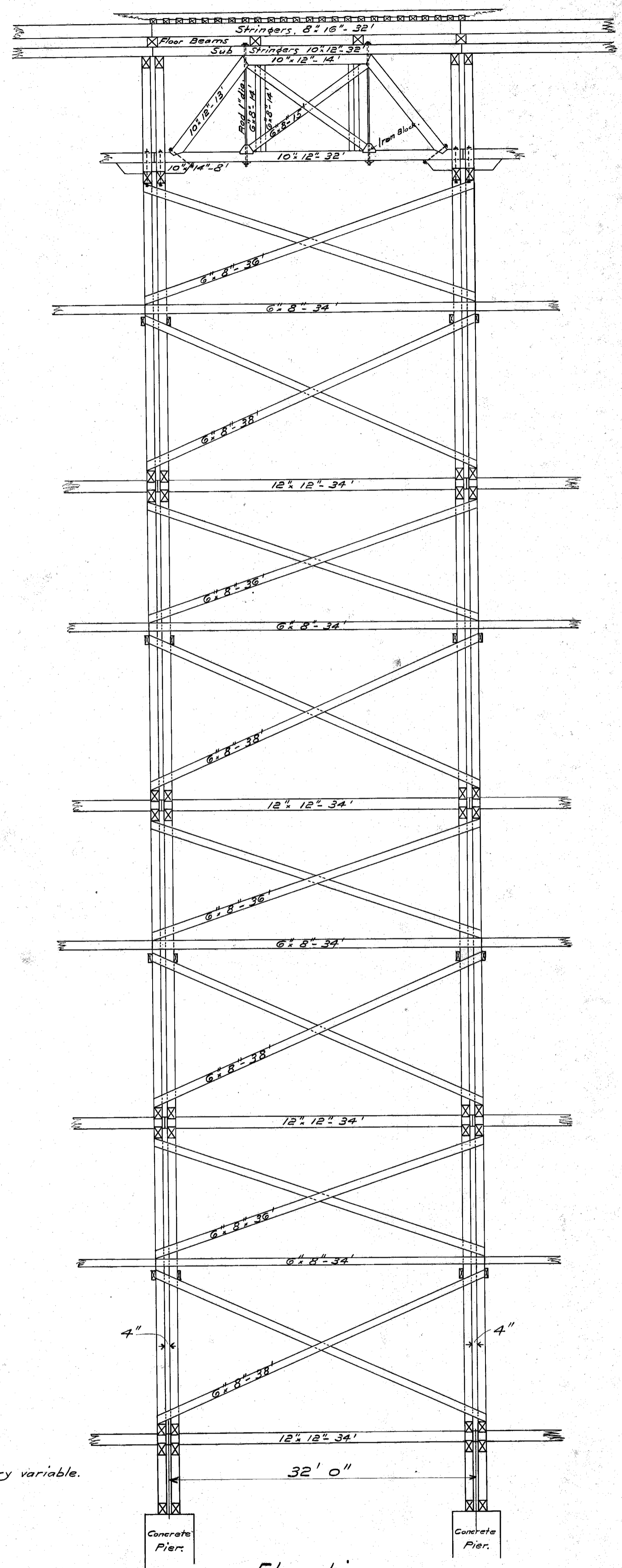
Elevation.
