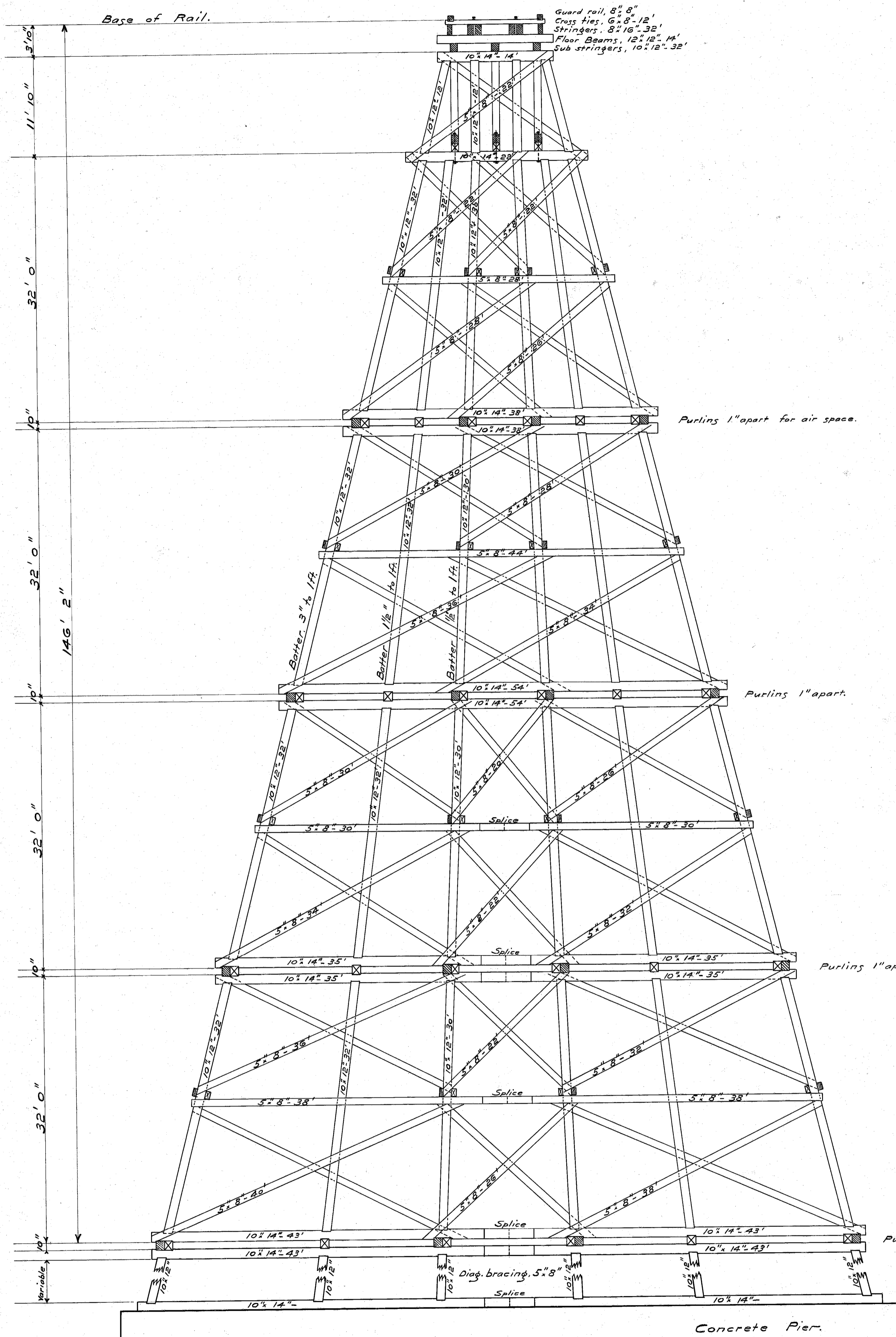
Elevation of Bent.
