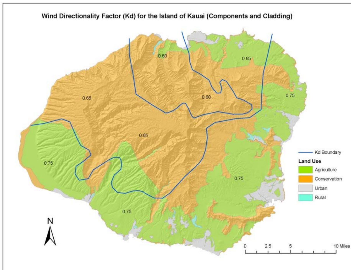
Figure 1609.3.4(b)(4)
