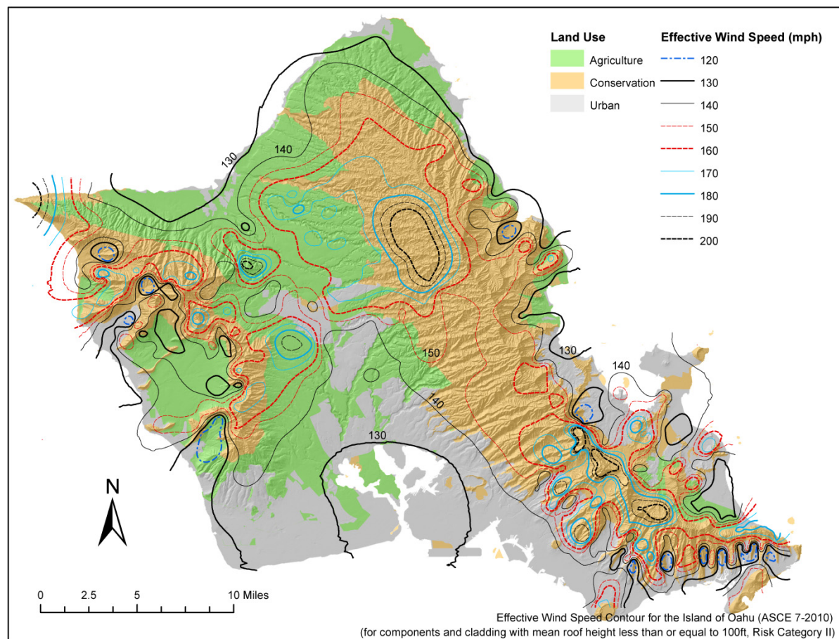
Figure 1609.3.2.2(e) City and County of Honolulu Effective Ultimate Wind Speed, V_{eff-ult} , for Components and Cladding for Risk Category II Buildings less than 100 feet Tall
