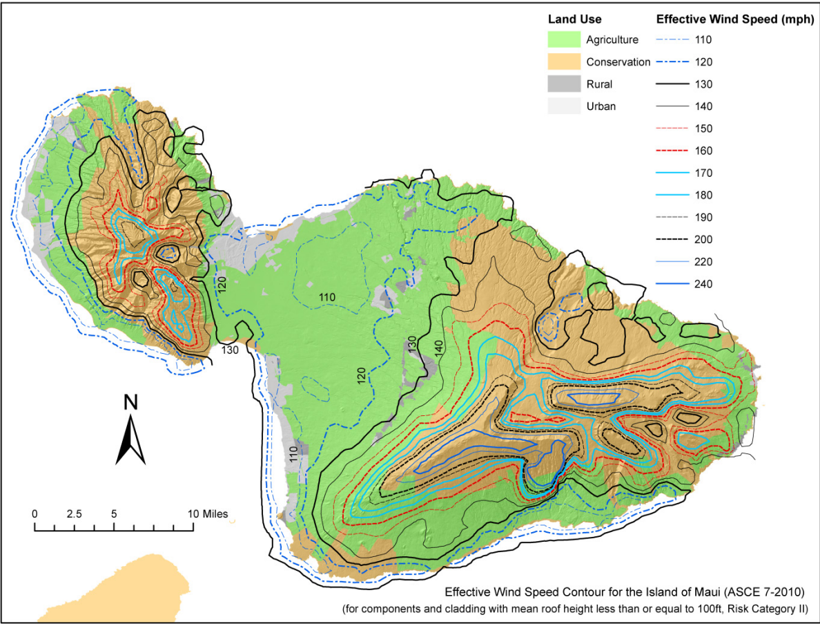
Figure 1609.3.2.1(b) County of Maui, Island of Maui Effective Ultimate Wind Speed, V_{eff-ult} , for Components and Cladding for Risk Category II Buildings less than 100 feet Tall
