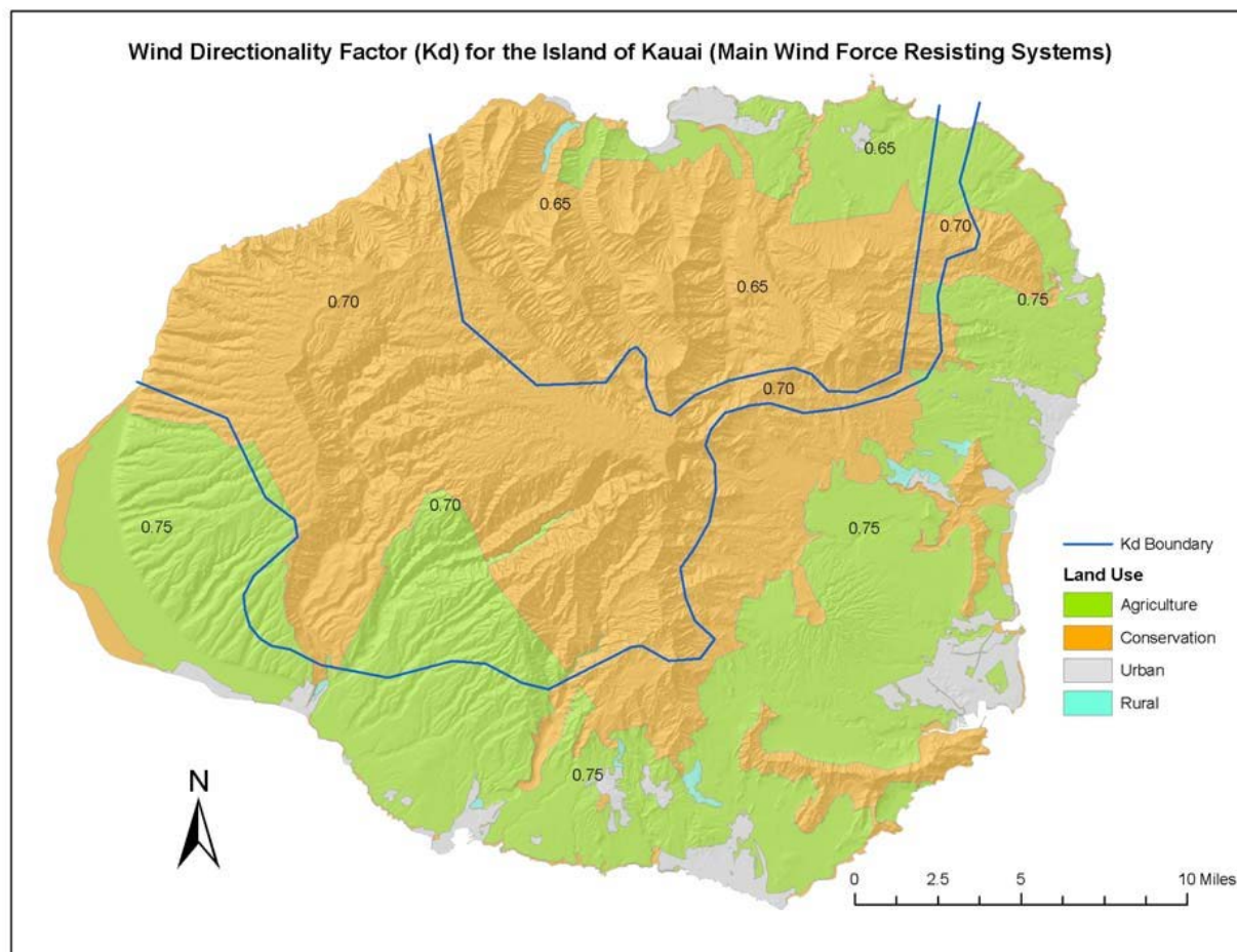
Figure 1609.3.4(a)(4)
