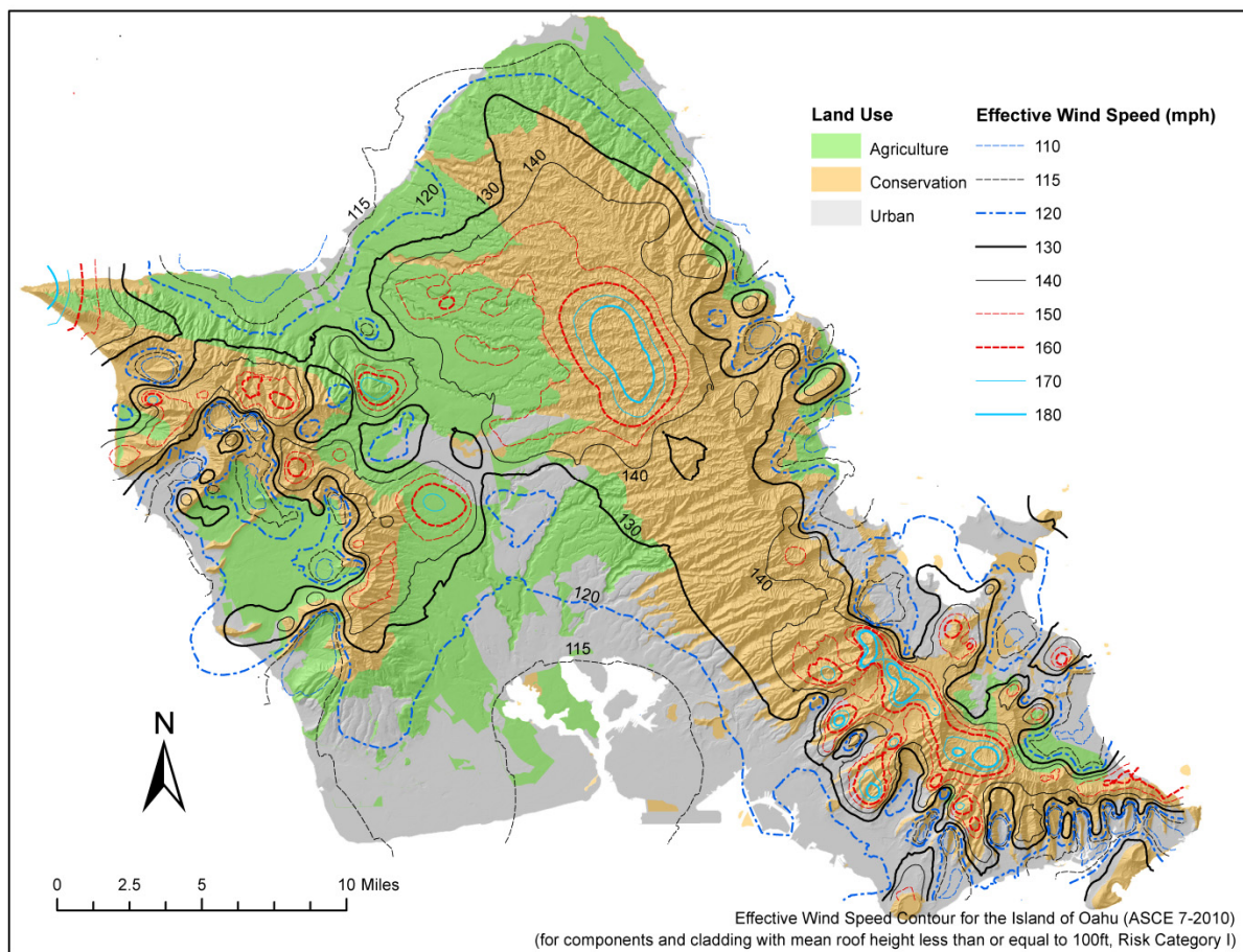
Figure 1609.3.2.1(e) City and County of Honolulu Effective Ultimate Wind Speed, V_{eff-ult} , for Components and Cladding for Risk Category I Buildings less than 100 feet Tall
