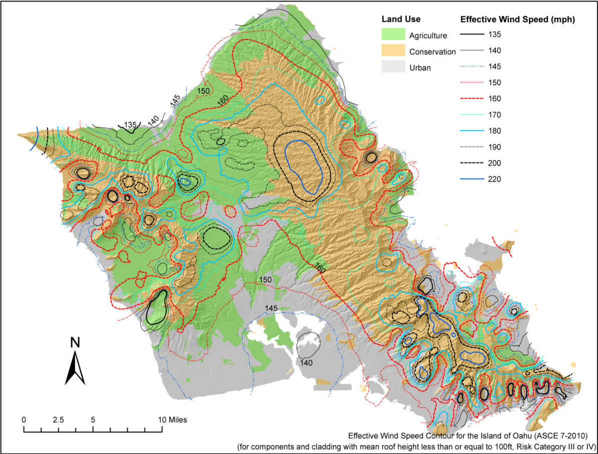
Figure 1609.3.2.3(e) City and County of Honolulu Effective Ultimate Wind Speed, V_{eff-ult} , for Components and Cladding for Risk Category III and IV Buildings less than 100 feet Tall
