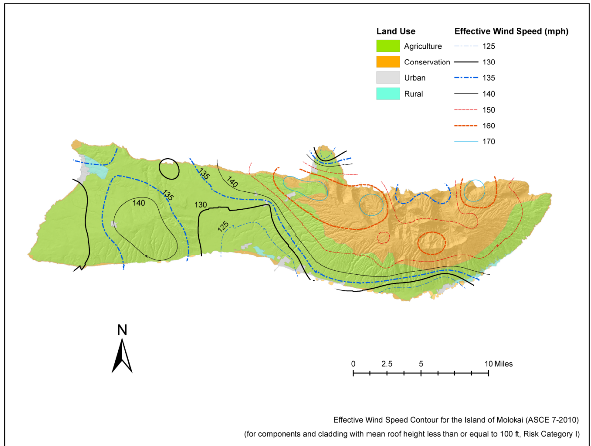
Figure 1609.3.2.1(c) County of Maui, Island of Molokai Effective Ultimate Wind Speed, V_{eff-ult} , for Components and Cladding for Risk Category I Buildings less than 100 feet Tall
