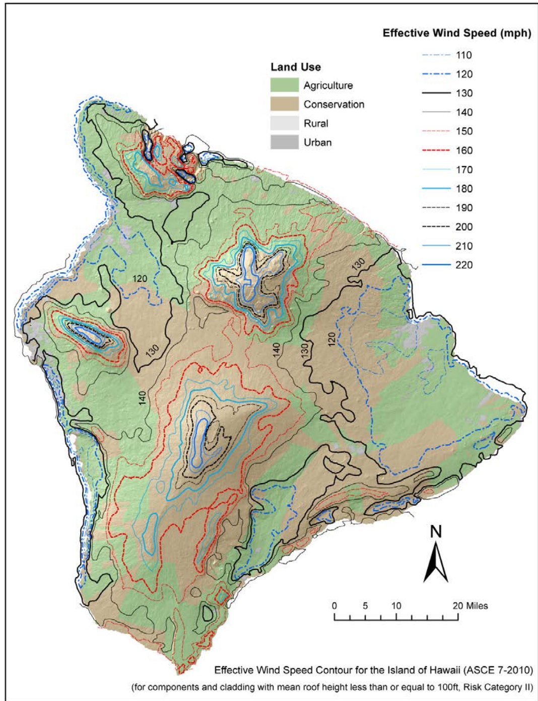
Figure 1609.3.2.2(a) County of Hawaii Effective Ultimate Wind Speed, V_{eff-ult} , for Components and Cladding for Risk Category II Buildings less than 100 feet Tall
