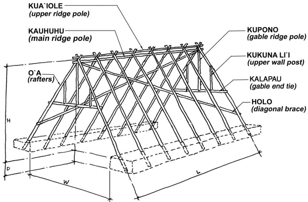
FRAMING SCHEMATIC
