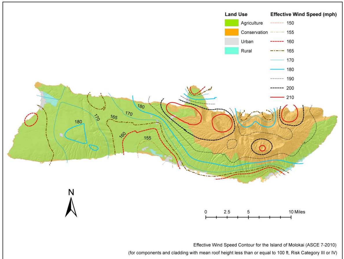
Figure 1609.3.2.3(c) County of Maui, Island of Molokai Effective Ultimate Wind Speed, V_{eff-ult} , for Components and Cladding for Risk Category III and IV Buildings less than 100 feet Tall
