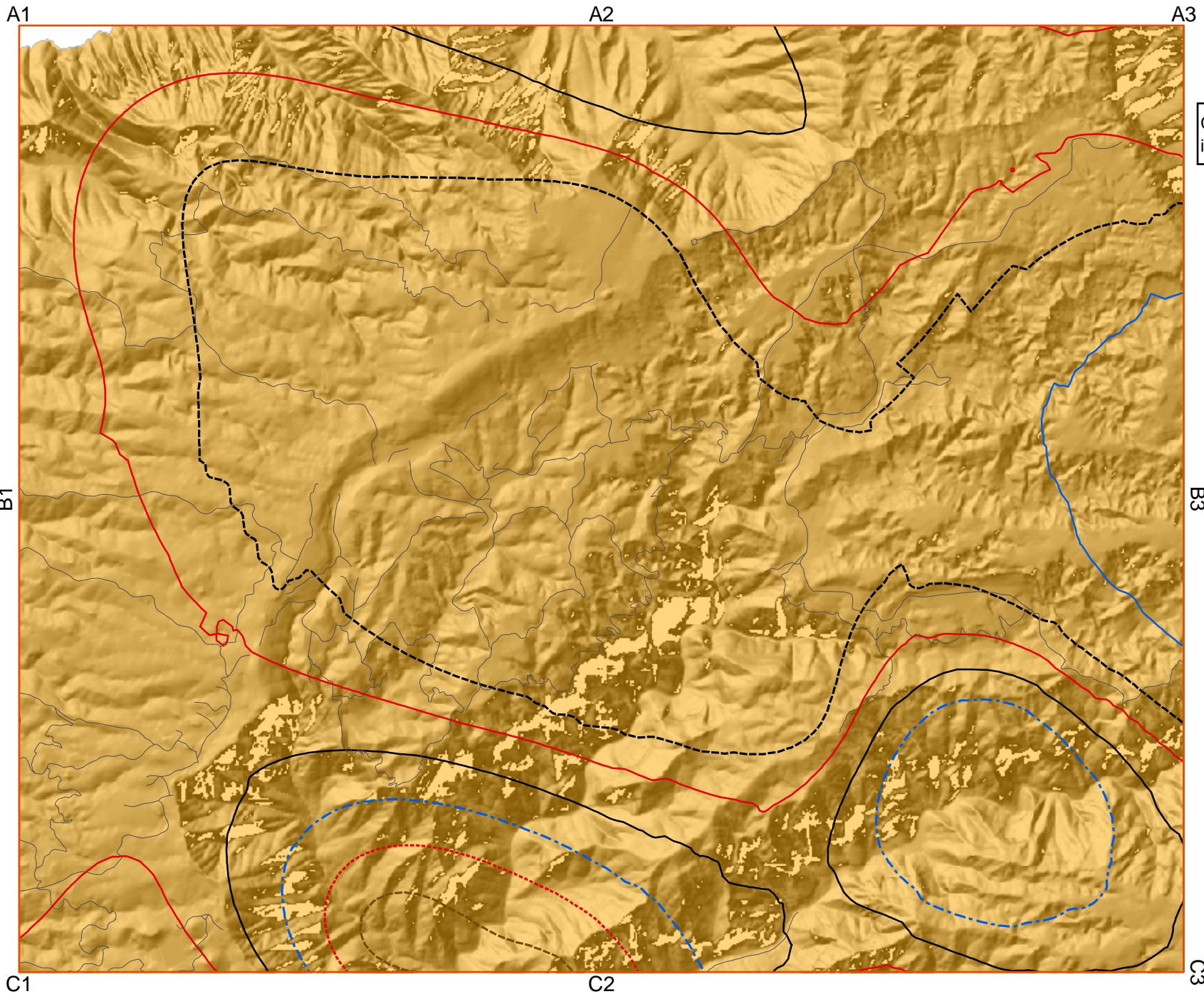
Wind Topographic Factor (Kzt) for the Island of Kauai (B2)
