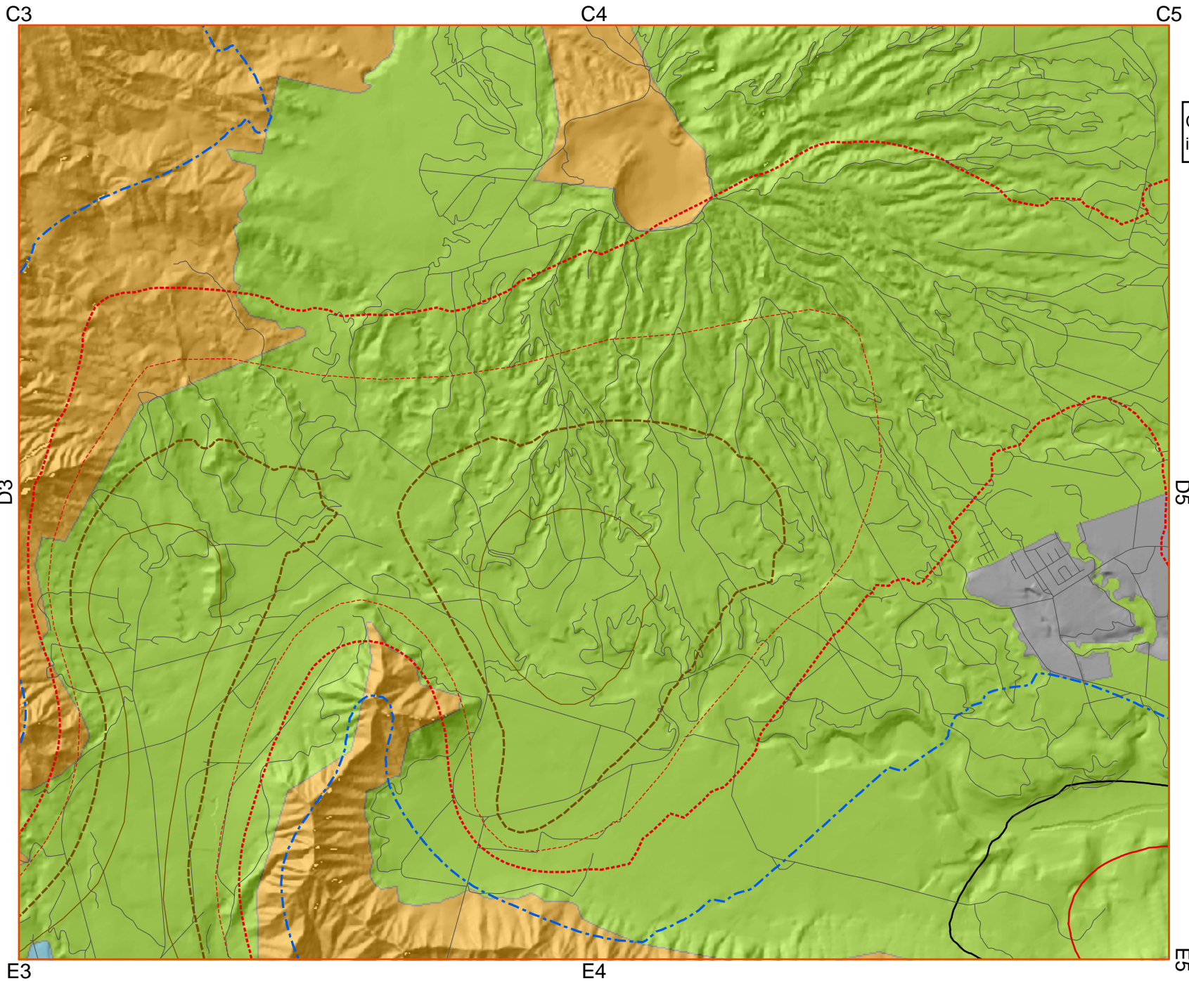
Wind Topographic Factor (Kzt) for the Island of Kauai (D4)
