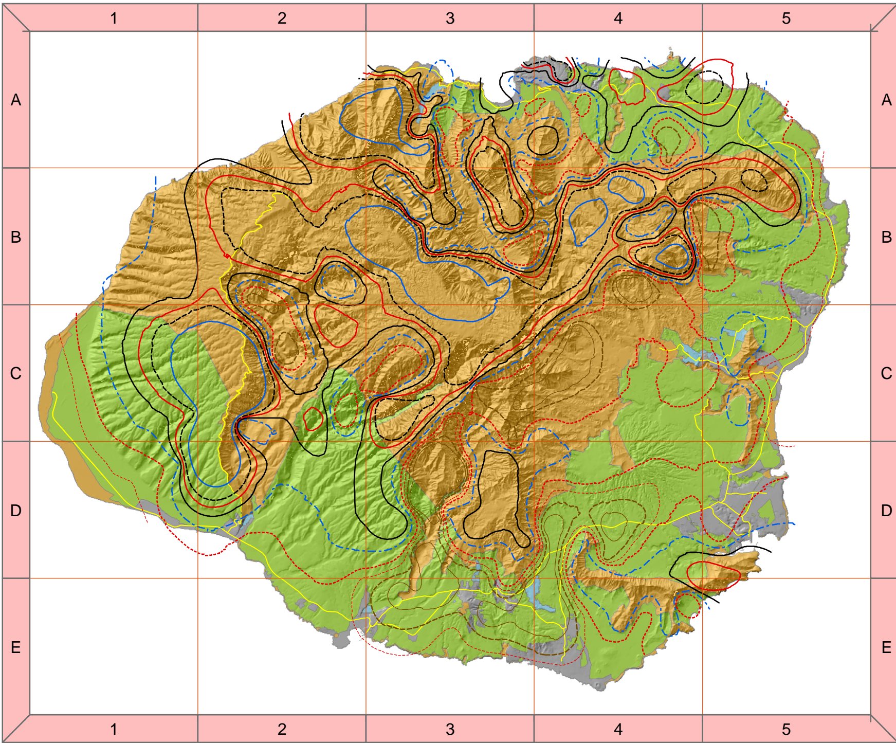
Wind Topographic Factor (Kzt) for the Island of Kauai
