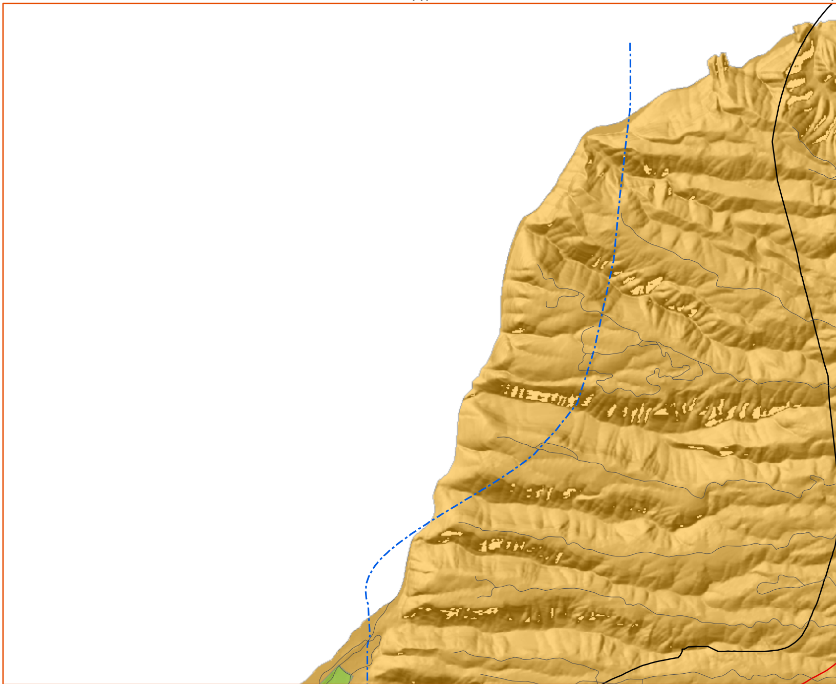
Wind Topographic Factor (Kzt) for the Island of Kauai (B1)
