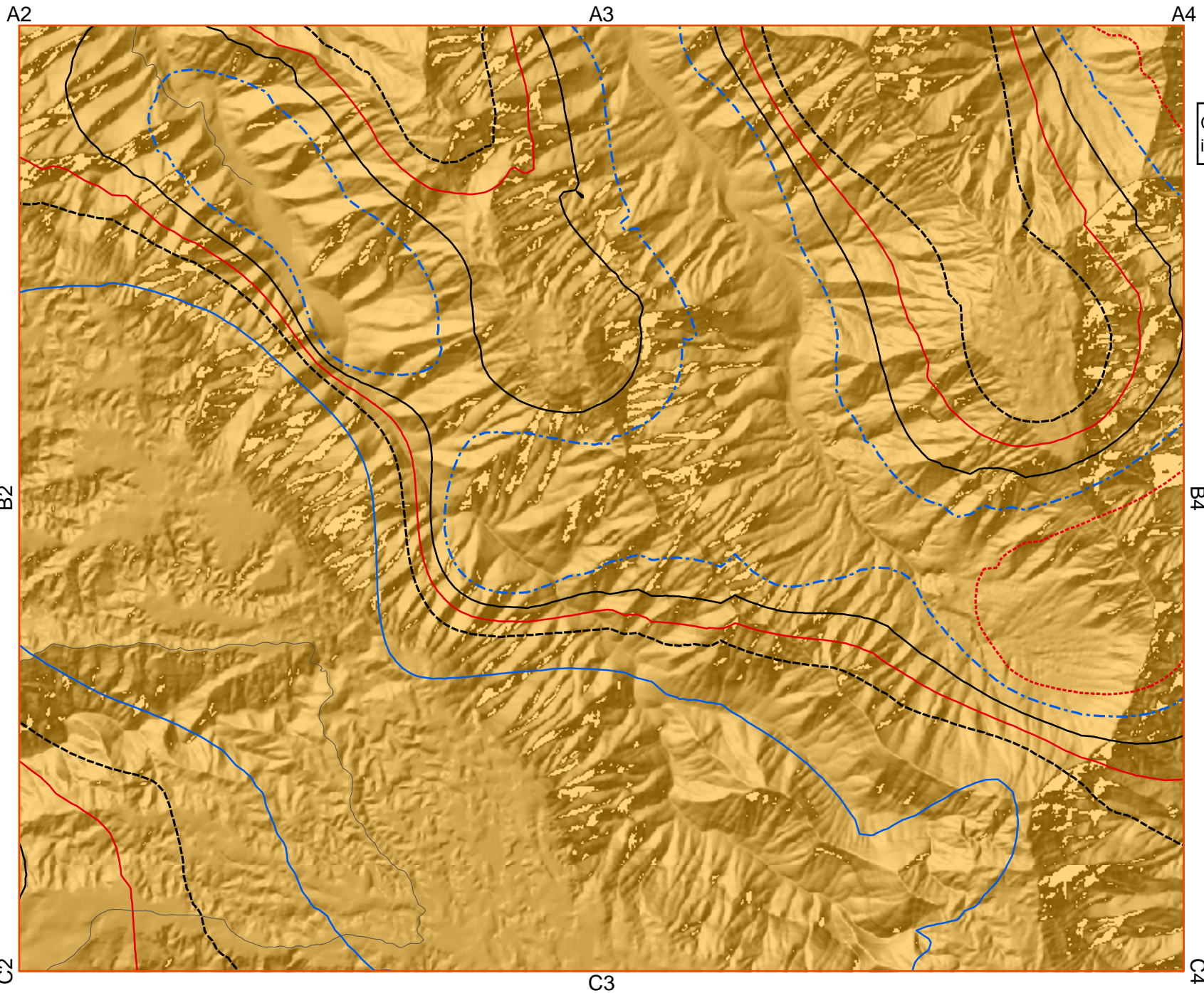
Wind Topographic Factor (Kzt) for the Island of Kauai (B3)
