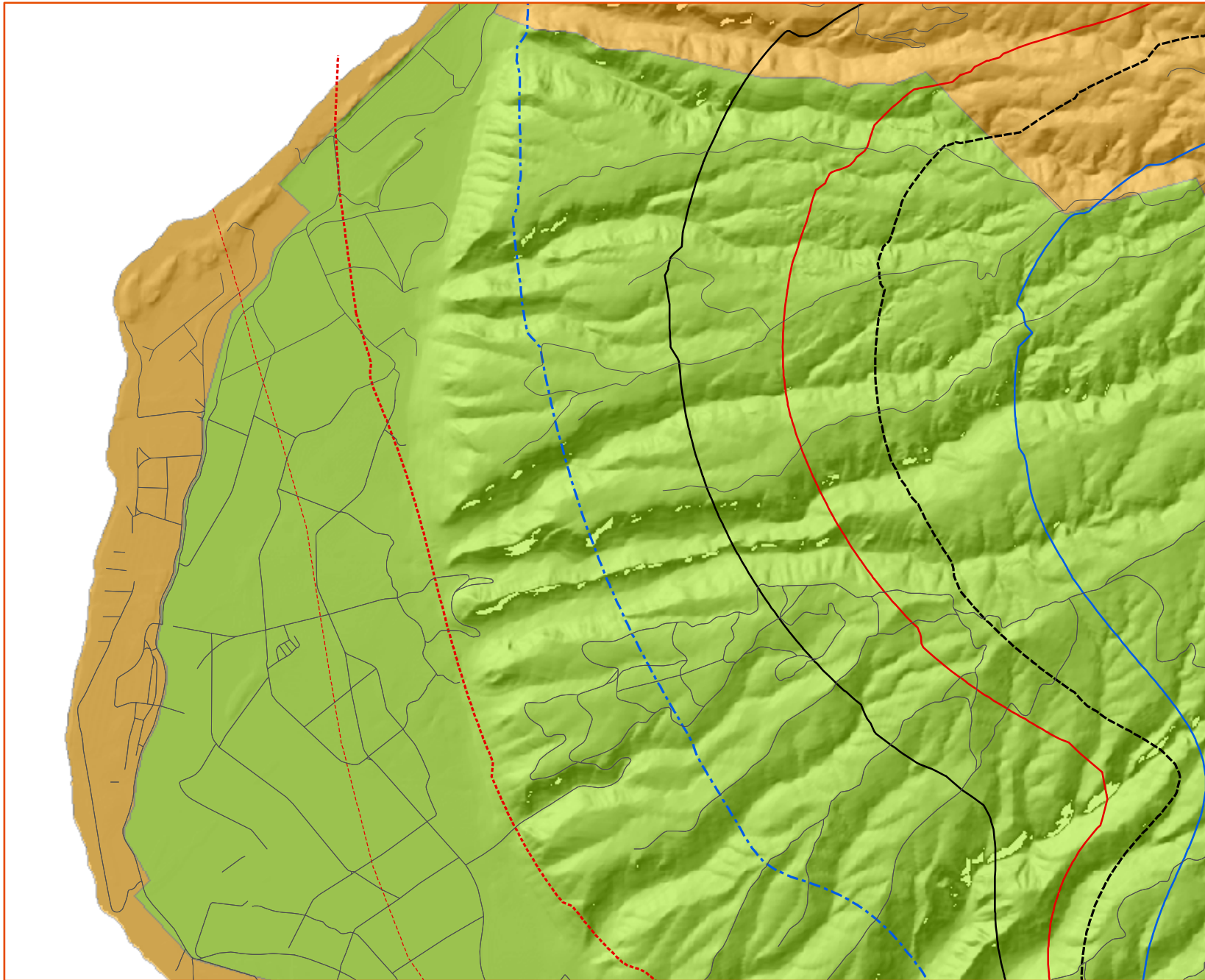
Wind Topographic Factor (Kzt) for the Island of Kauai (C1)
