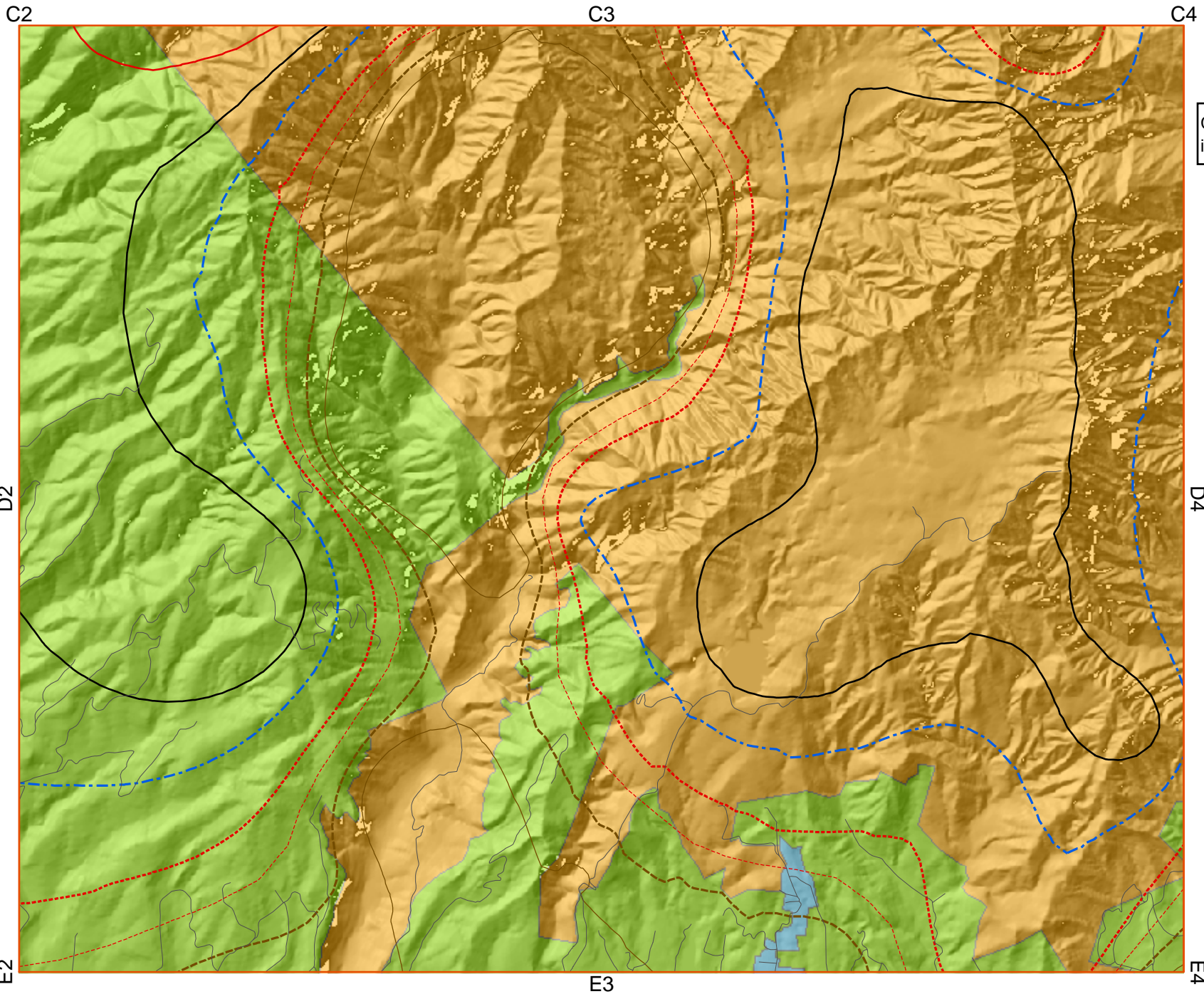
Wind Topographic Factor (Kzt) for the Island of Kauai (D3)
