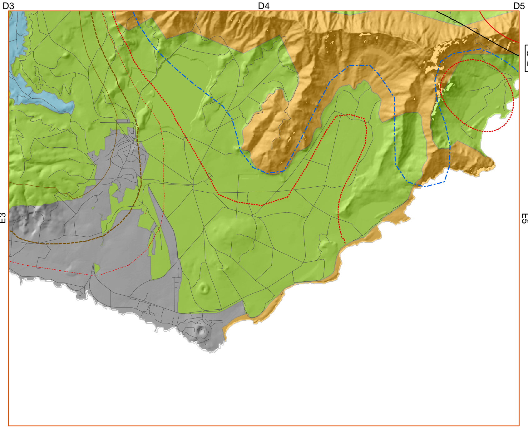
Wind Topographic Factor (Kzt) for the Island of Kauai (E4)
