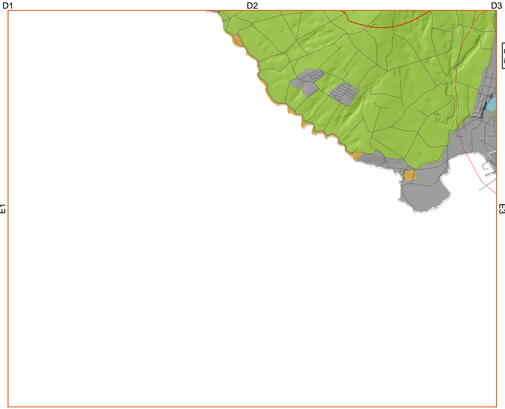
Wind Topographic Factor (Kzt) for the Island of Kauai (E2)
