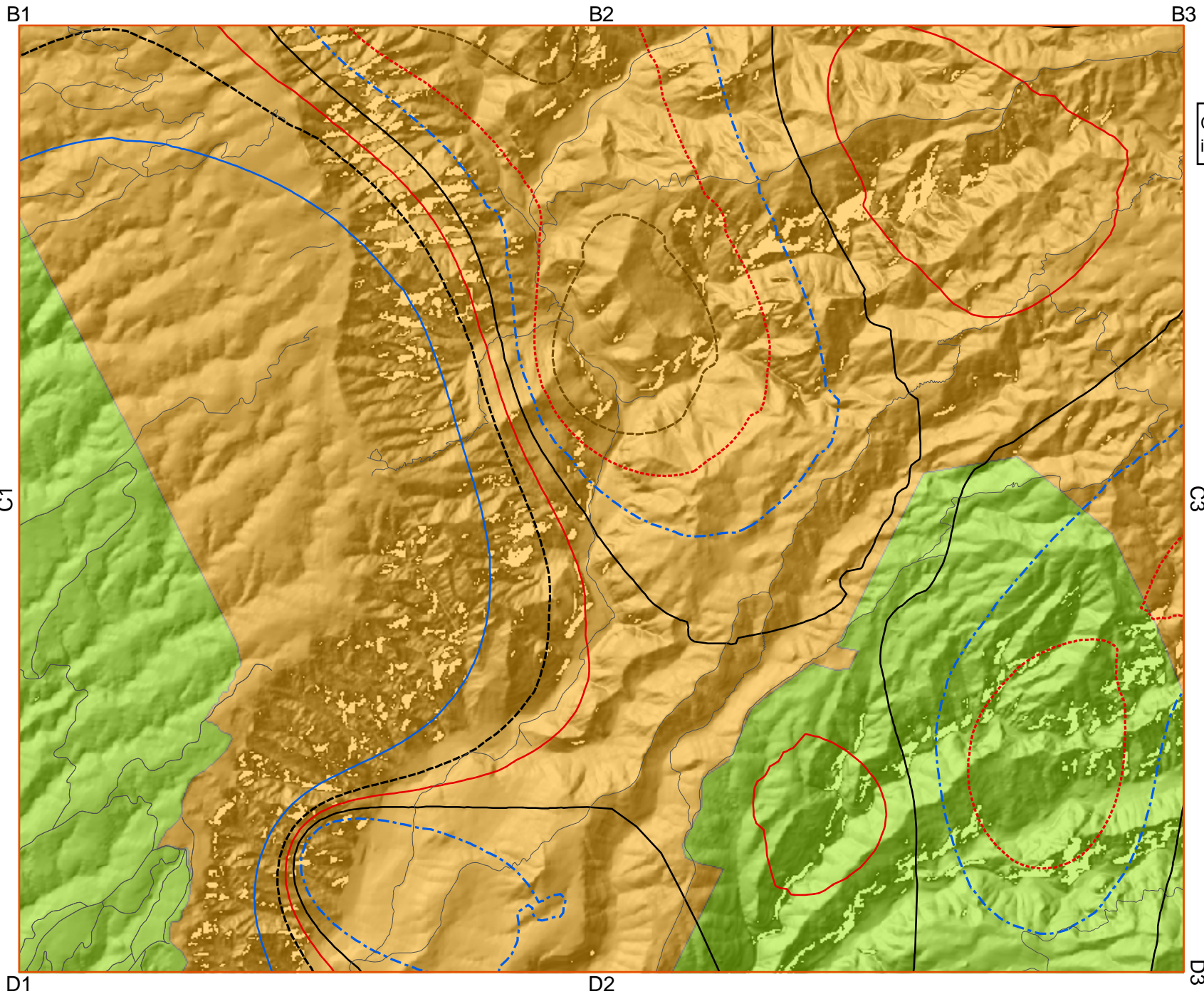
Wind Topographic Factor (Kzt) for the Island of Kauai (C2)
