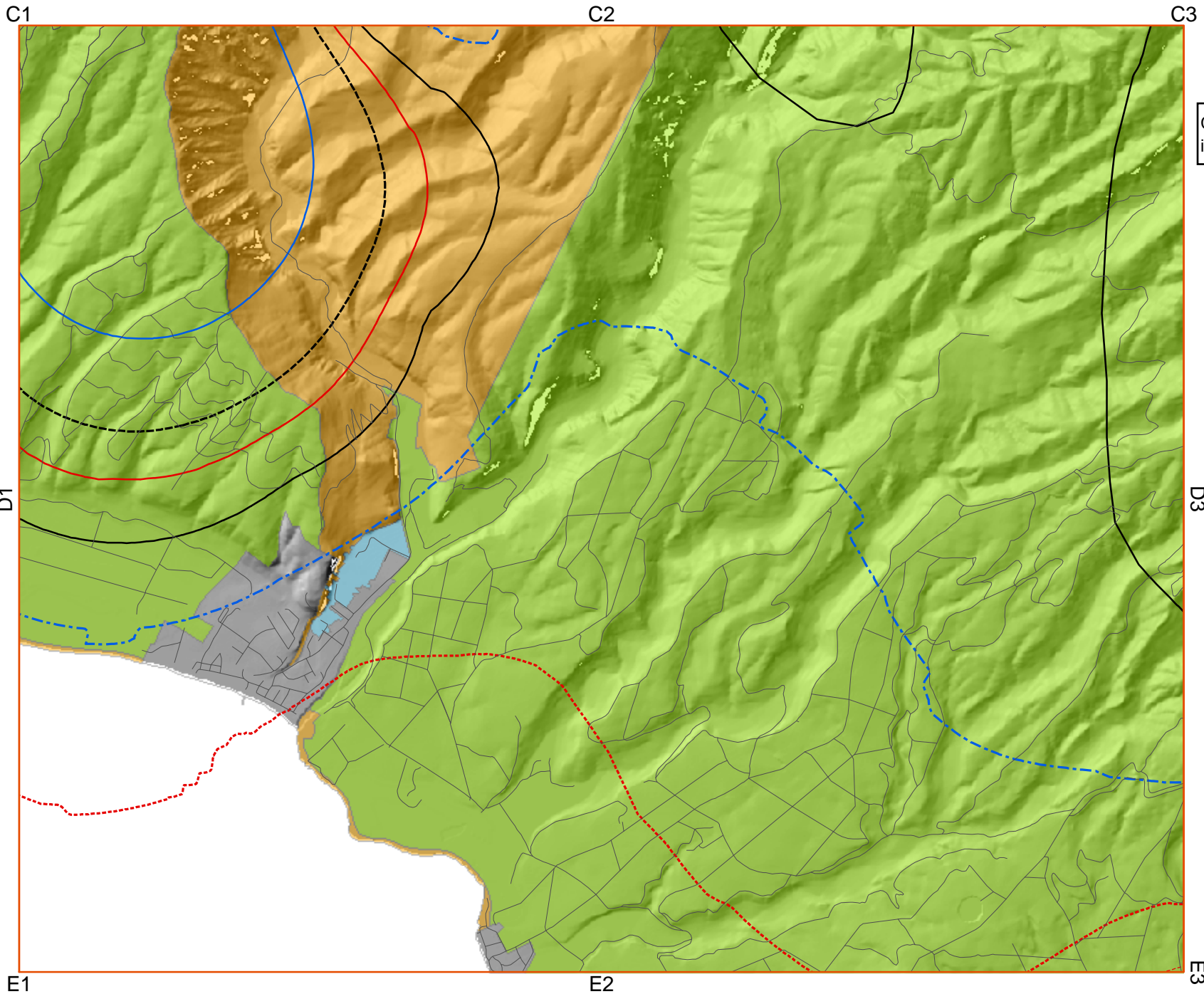
Wind Topographic Factor (Kzt) for the Island of Kauai (D2)
