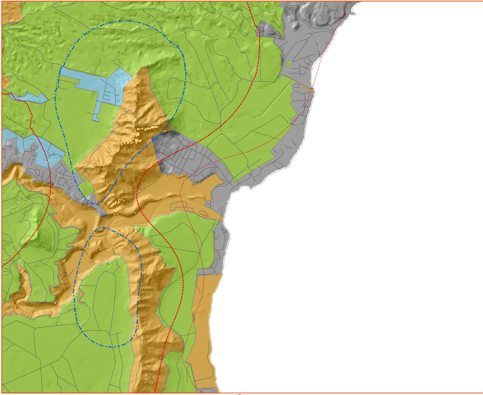
Wind Topographic Factor (Kzt) for the Island of Kauai (C5)
