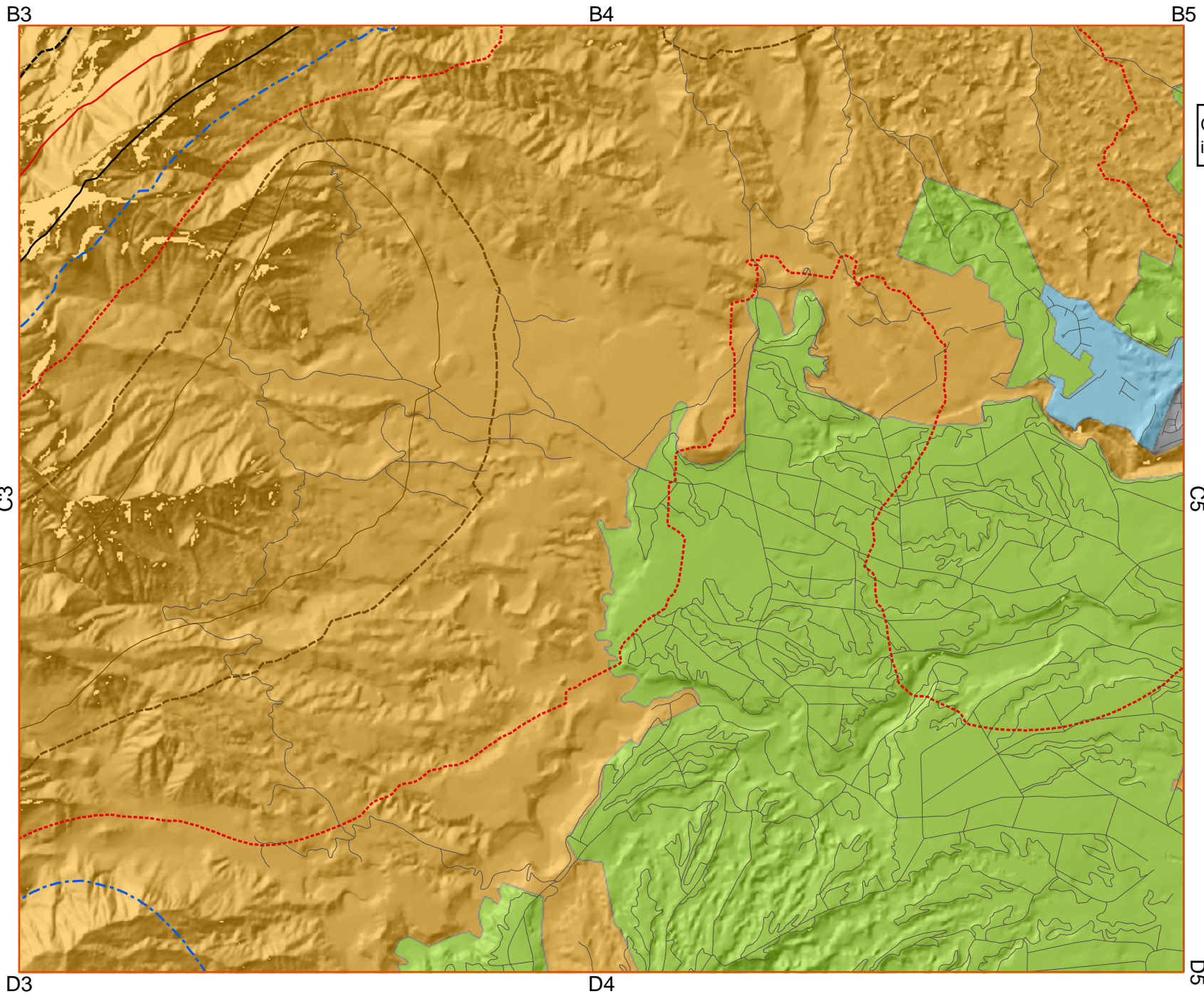
Wind Topographic Factor (Kzt) for the Island of Kauai (C4)
