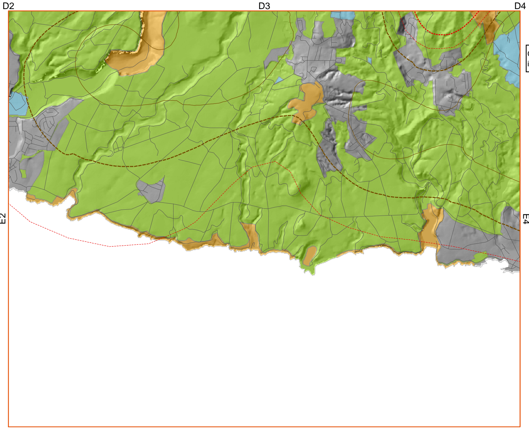
Wind Topographic Factor (Kzt) for the Island of Kauai (E3)
