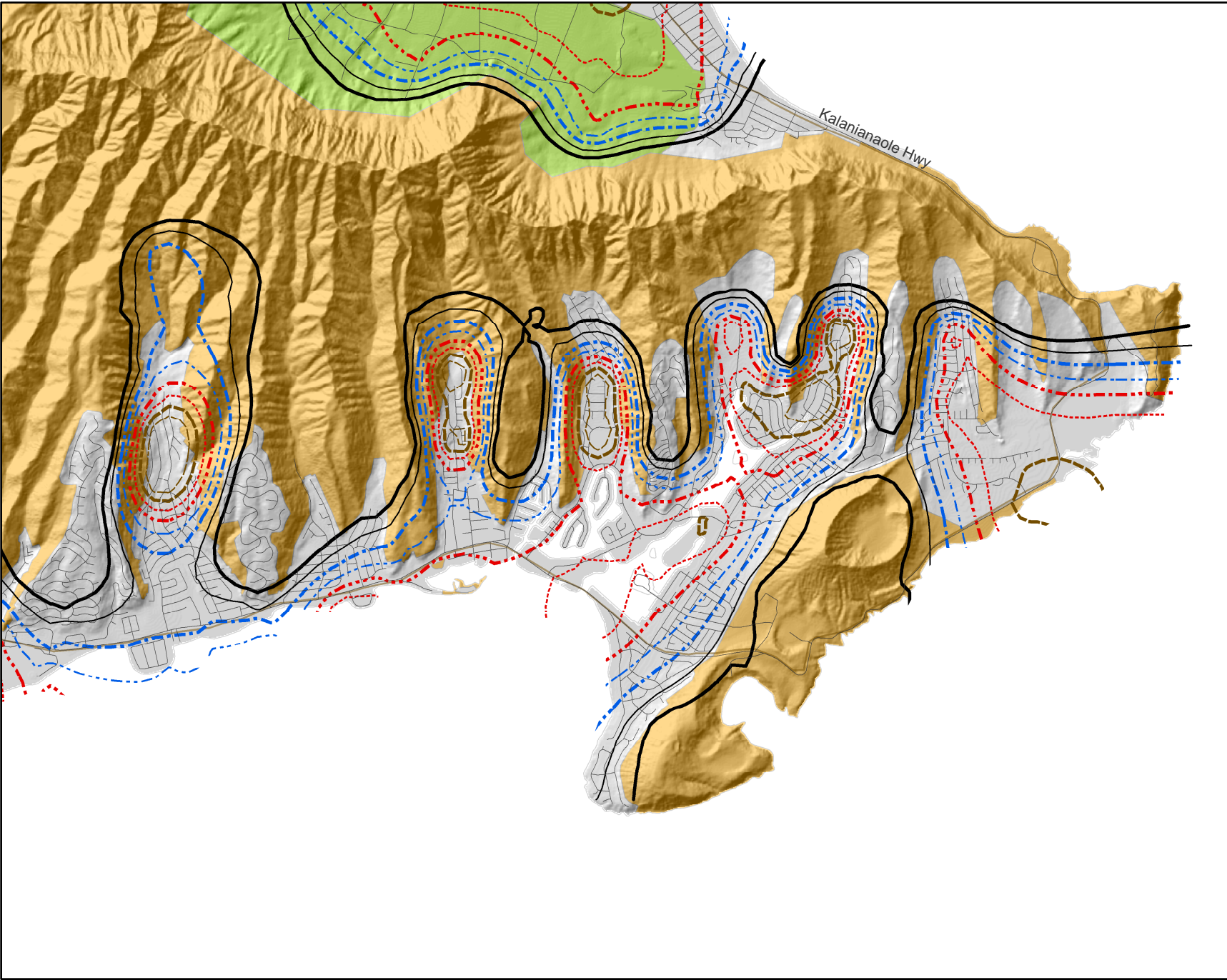
Kzt Contour for the Island of Oahu (E5)
