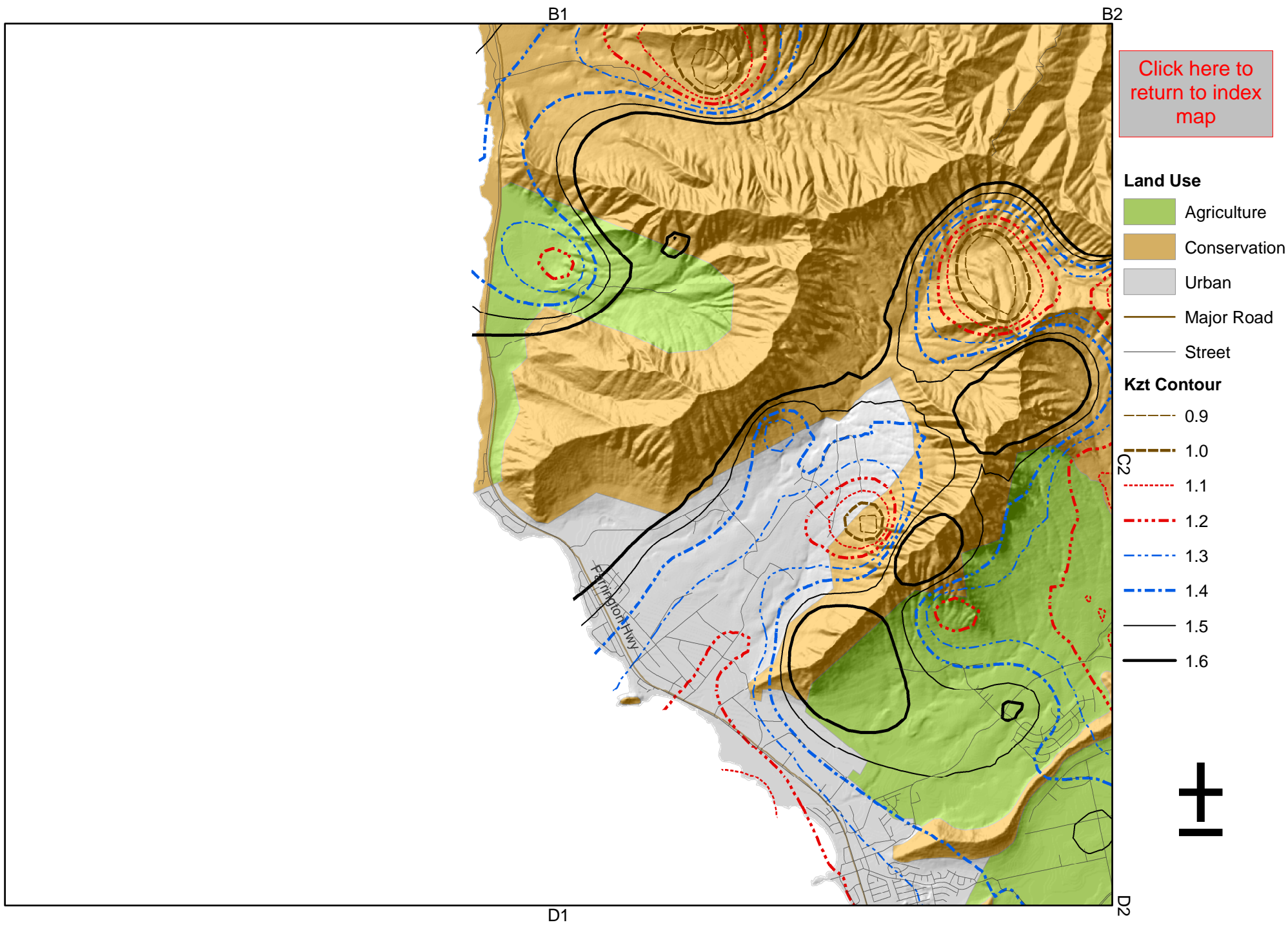
Kzt Contour for the Island of Oahu (C1)
