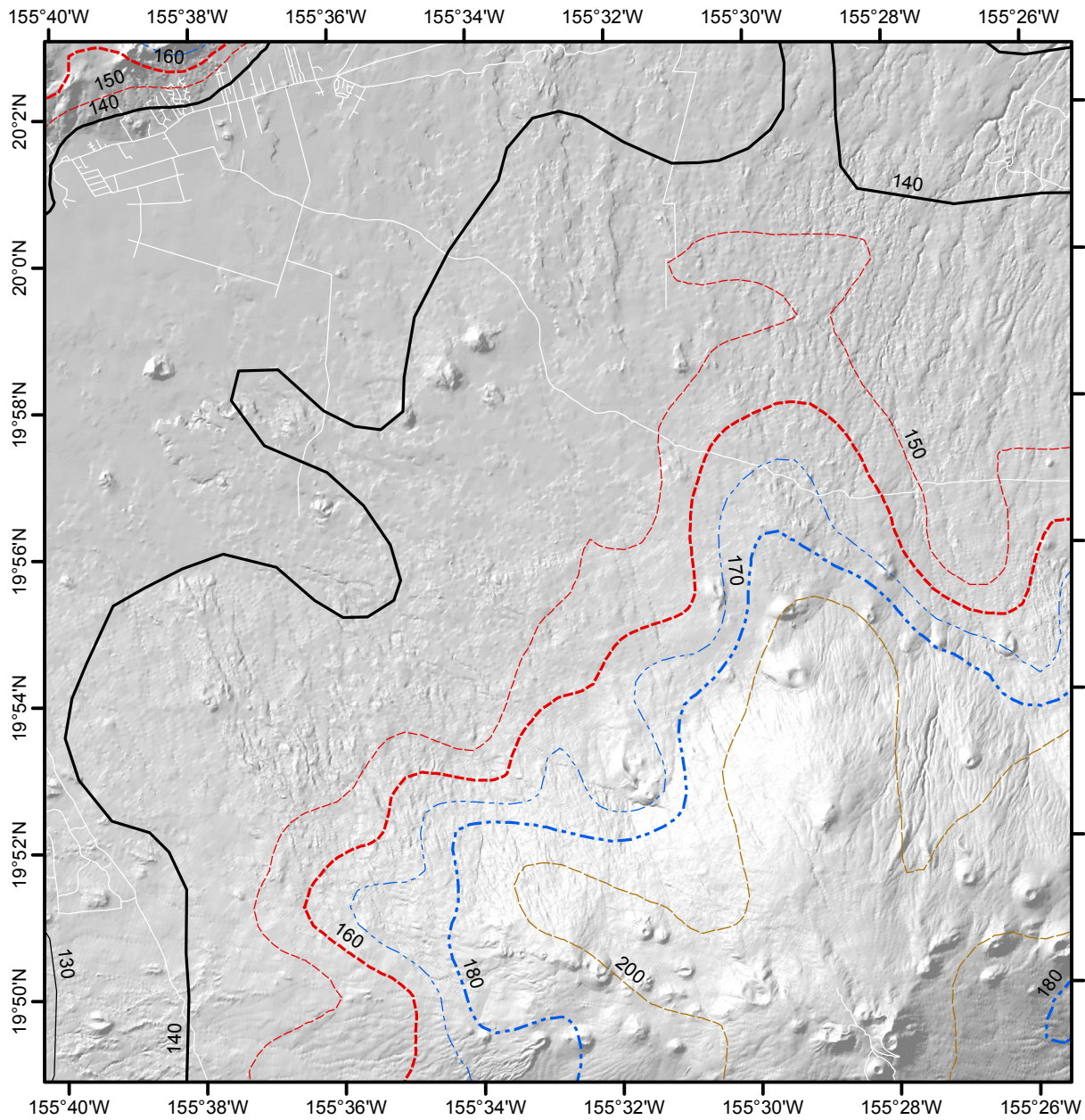
Figure R301.2(5)(a) County of Hawaii Ultimate Wind Speed, V_{ult} for Components and Cladding
