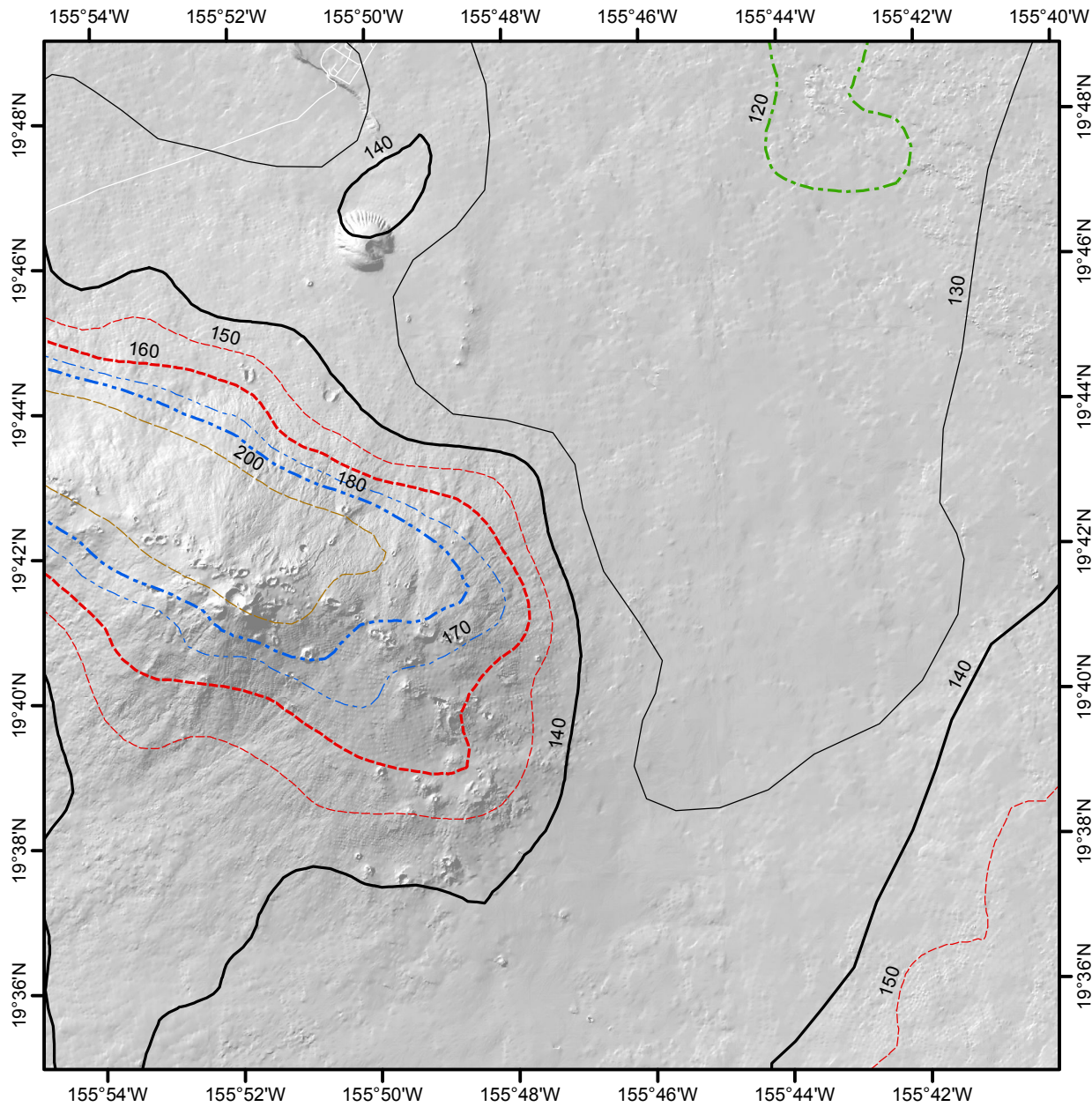
Figure R301.2(5)(a) County of Hawaii Ultimate Wind Speed, V_{ult} for Components and Cladding
