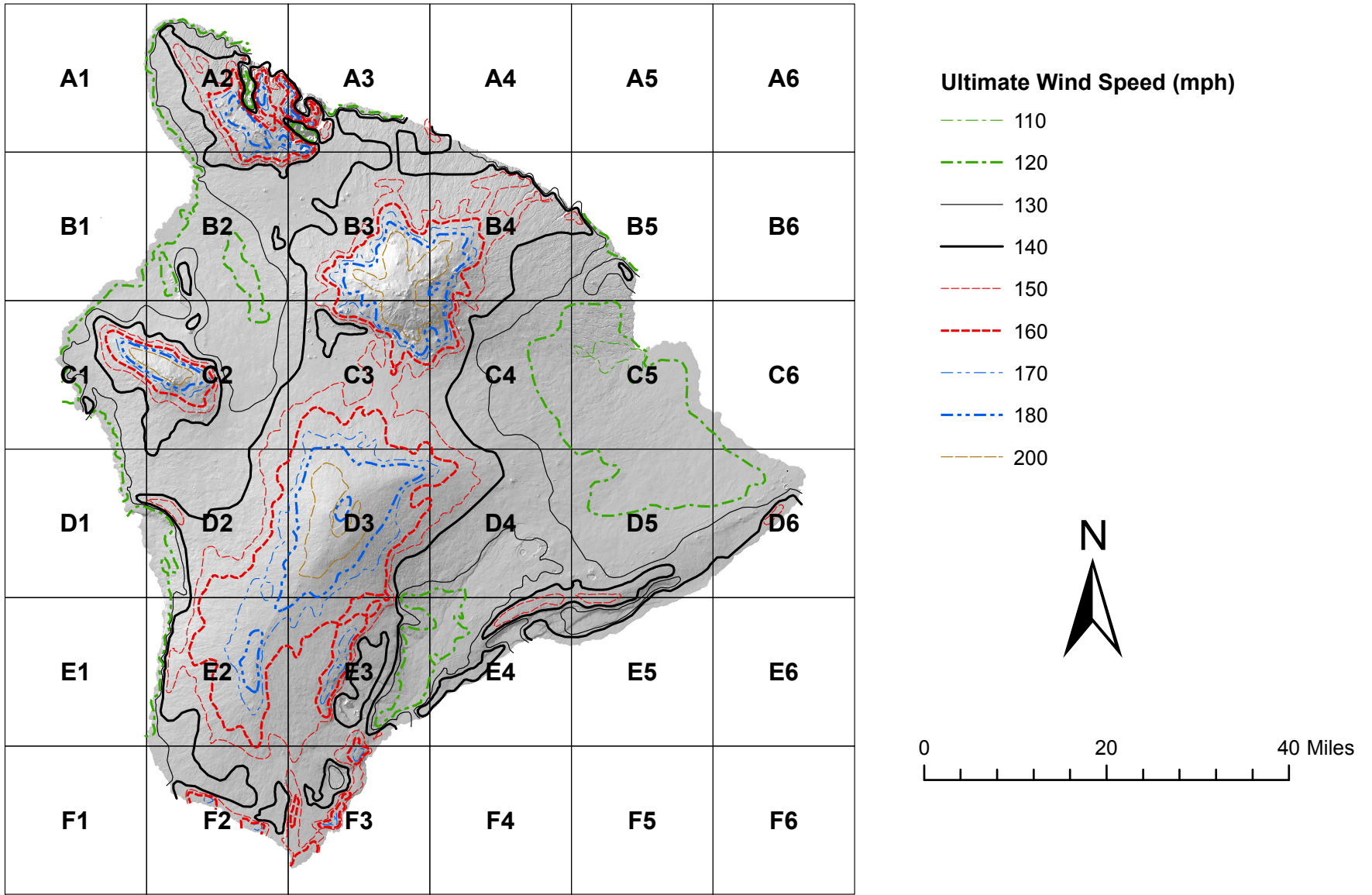
Figure R301.2(5)(a) County of Hawaii Ultimate Wind Speed, V_{ult} for Components and Cladding
