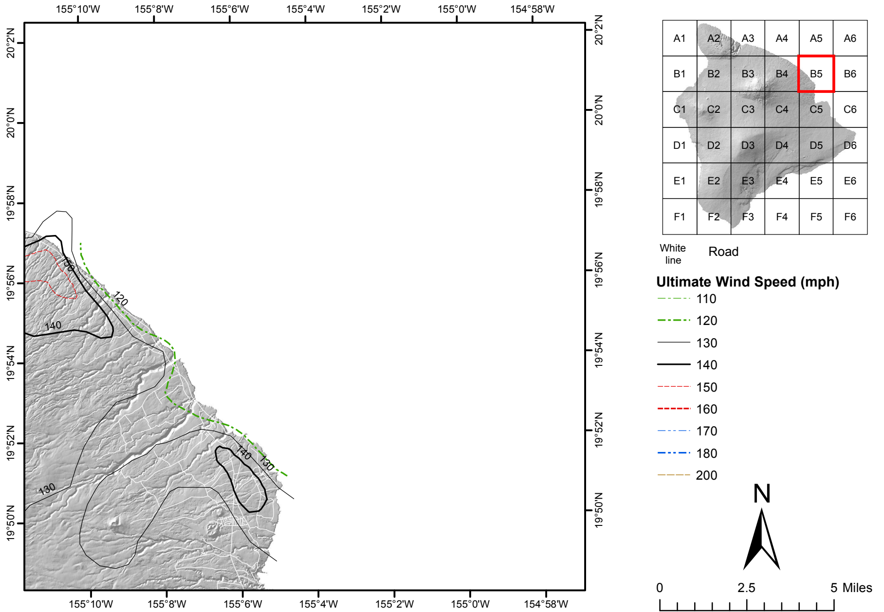
Figure R301.2(5)(a) County of Hawaii Ultimate Wind Speed, V_{ult} for Components and Cladding
